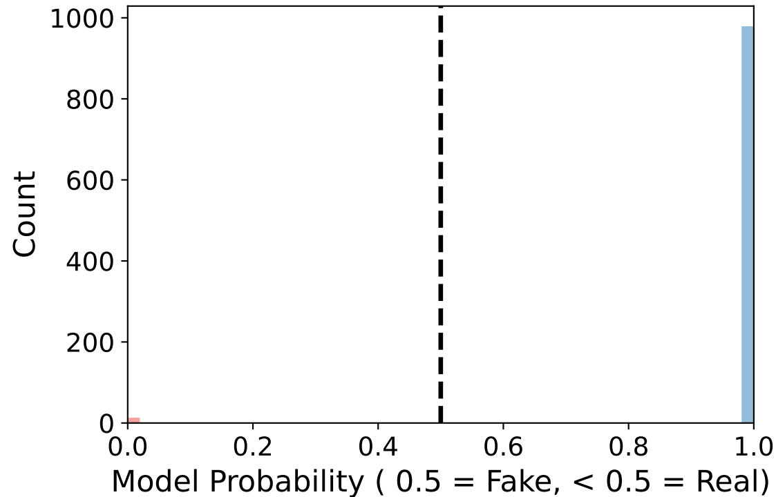
After PGD
