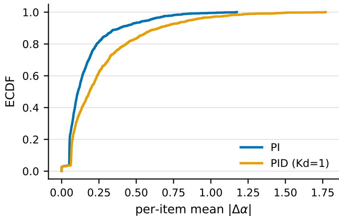
actuation roughness \text{mean}_t |\Delta\alpha(t)|
