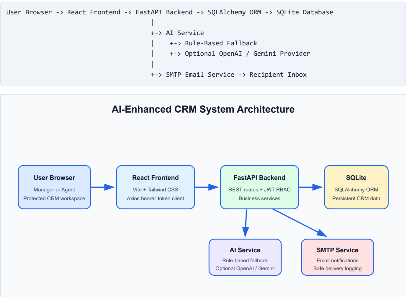
Figure 2. High-level architecture of the AI-enhanced CRM system.
