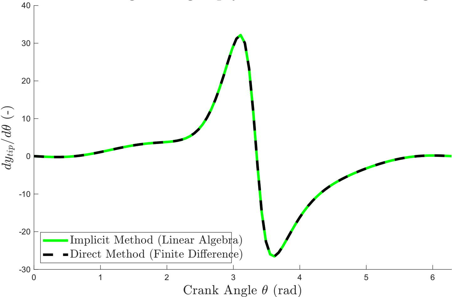
Rate of Change of Leg Tip y-Position with Crank Angle \theta
