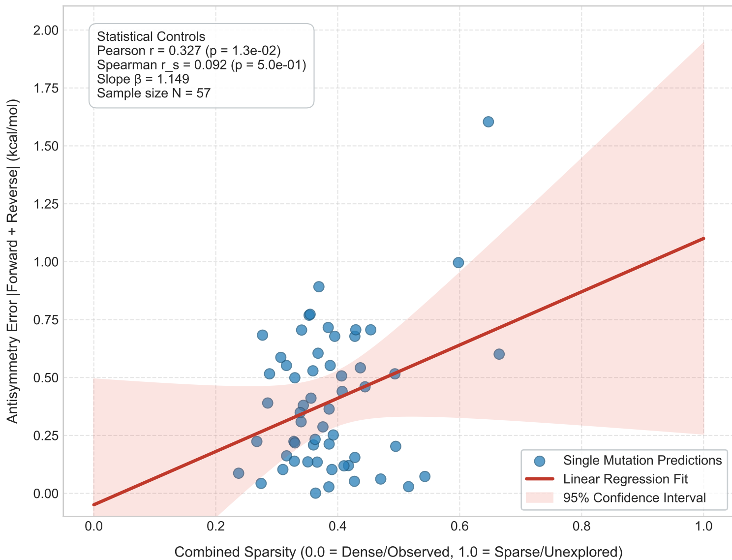
Figure F2: Thermodynamic Inconsistency vs. Mutation-Space Sparsity
