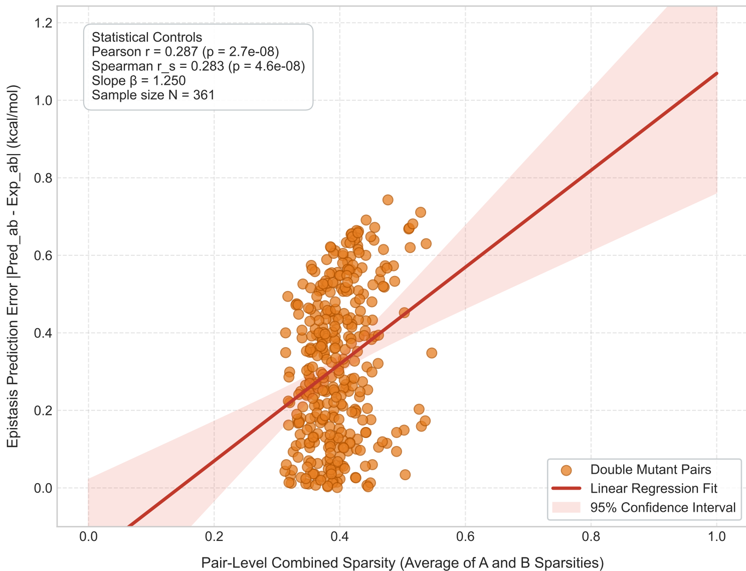
Figure F3: Epistasis Prediction Error vs. Mutation-Space Sparsity
