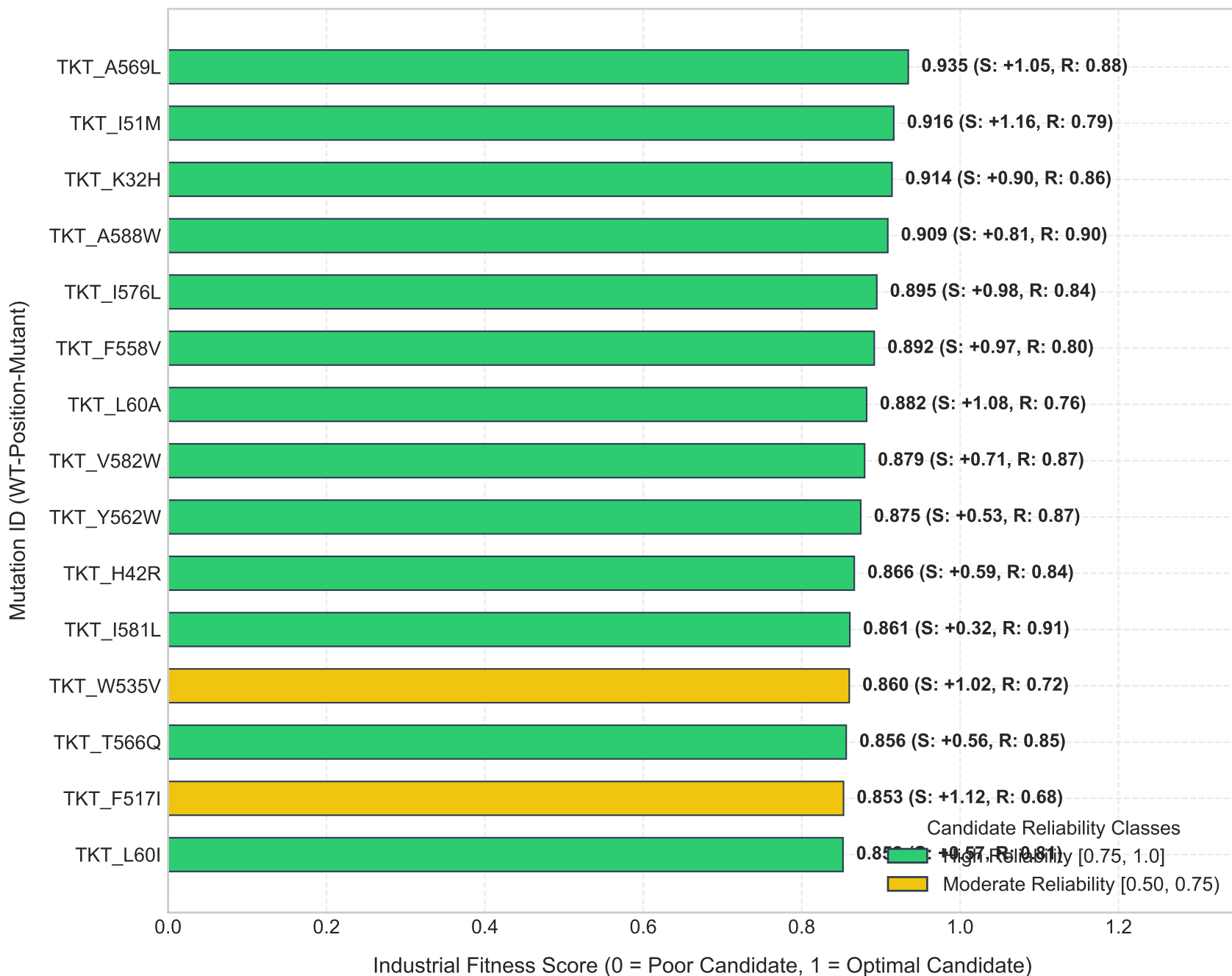
Figure F8: Top 15 Prioritized Transketolase Engineering Candidates
