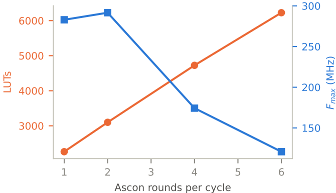
Faster mask expansion costs area and clock
