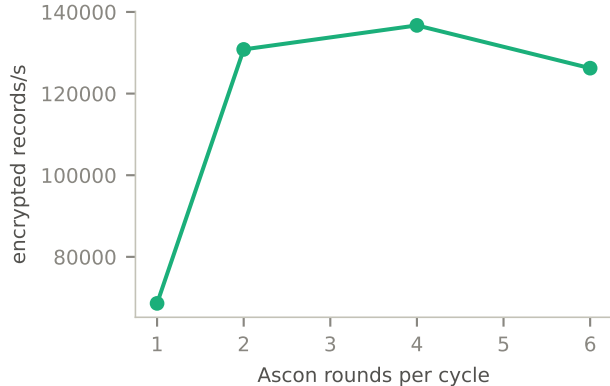
Real-time gain saturates
