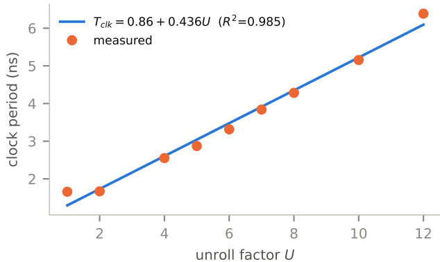
Critical path grows linearly with U
