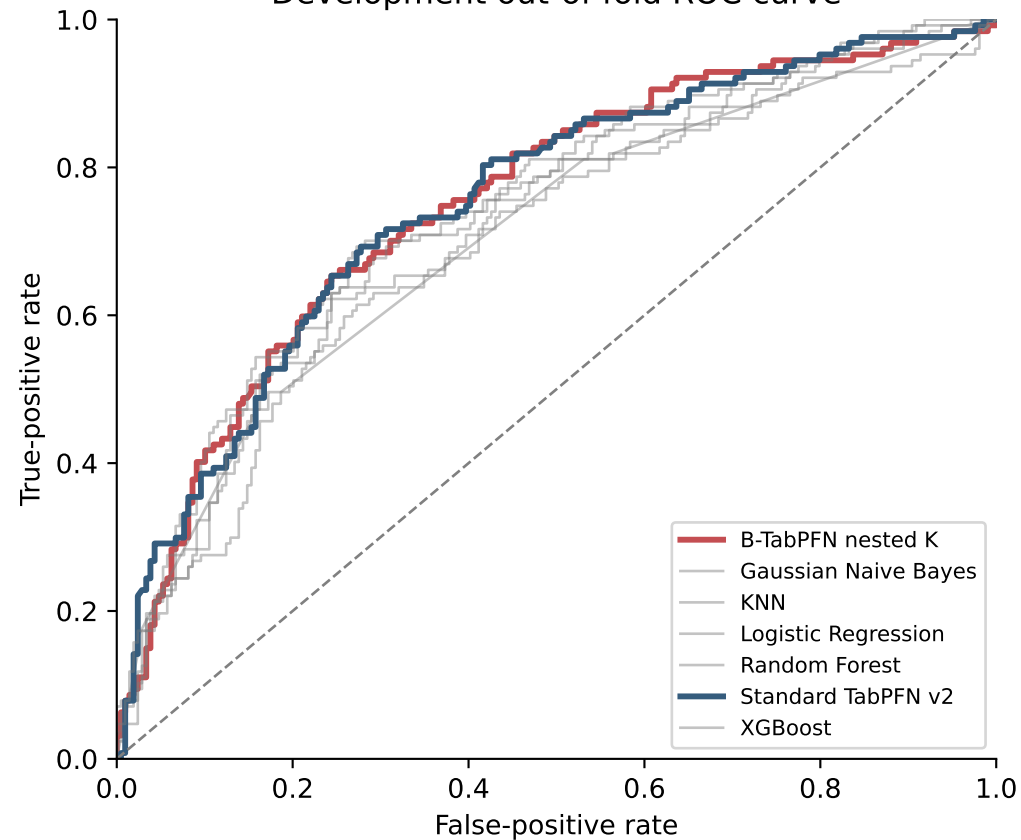
Development out-of-fold ROC curve
