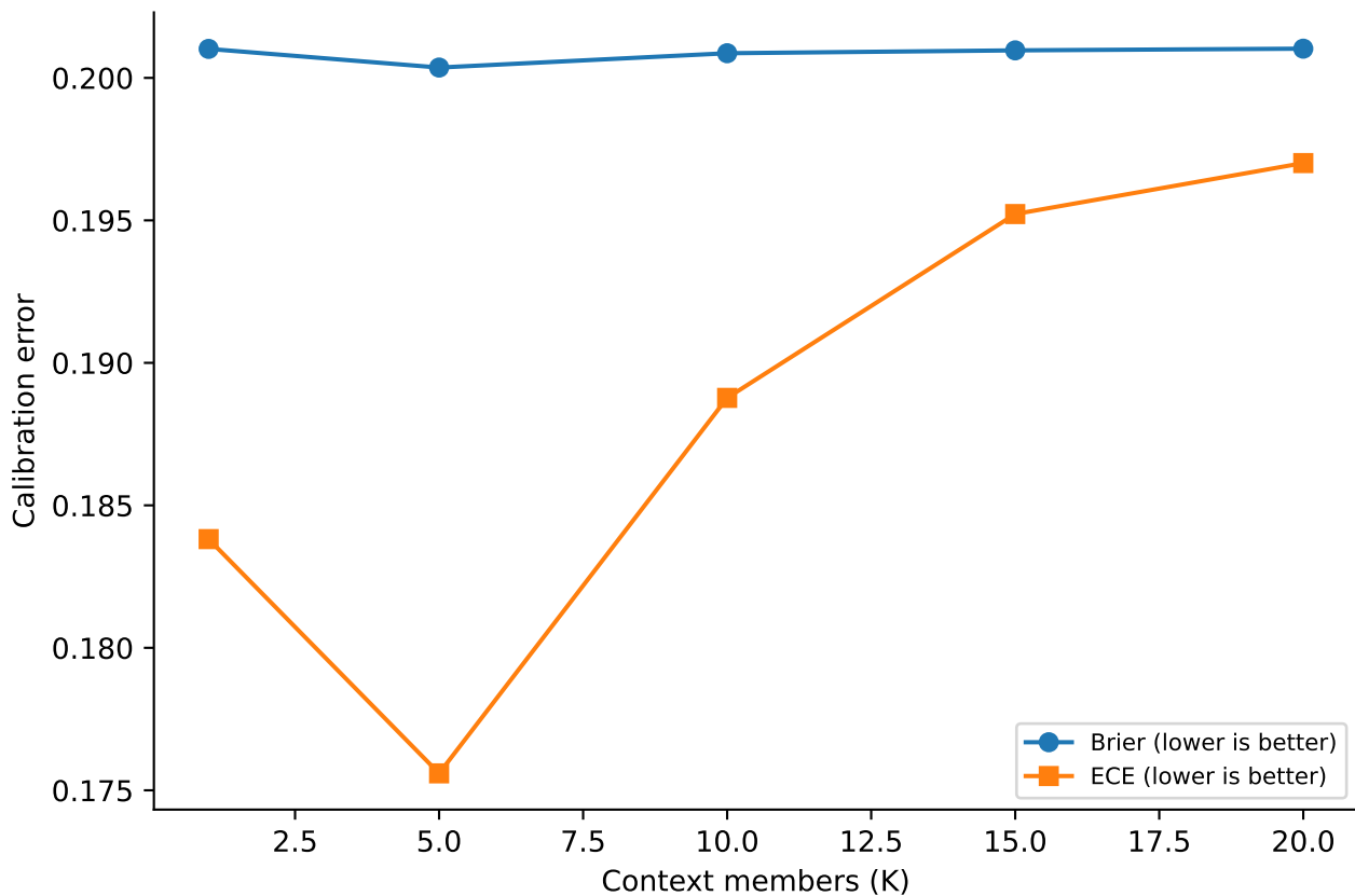
Calibration across K
