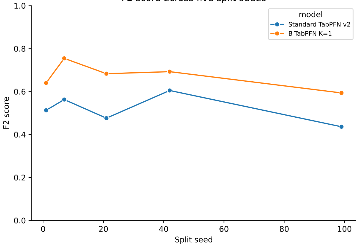
F2 score across five split seeds
