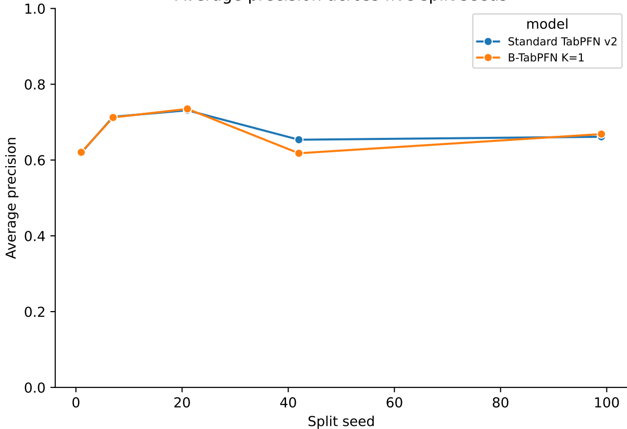
Average precision across five split seeds
