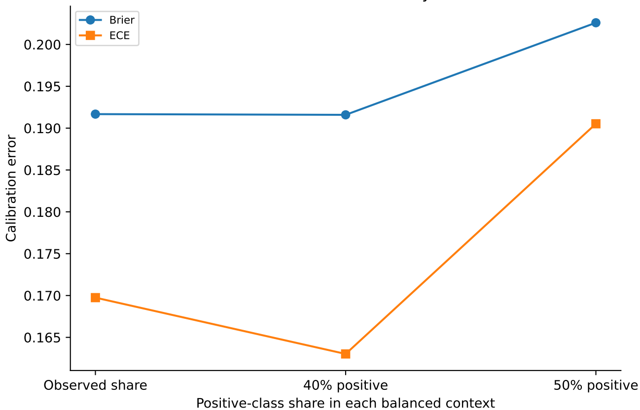
Calibration sensitivity
