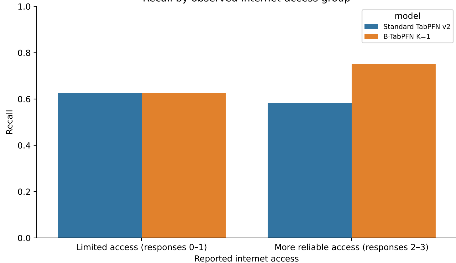
Recall by observed internet-access group
