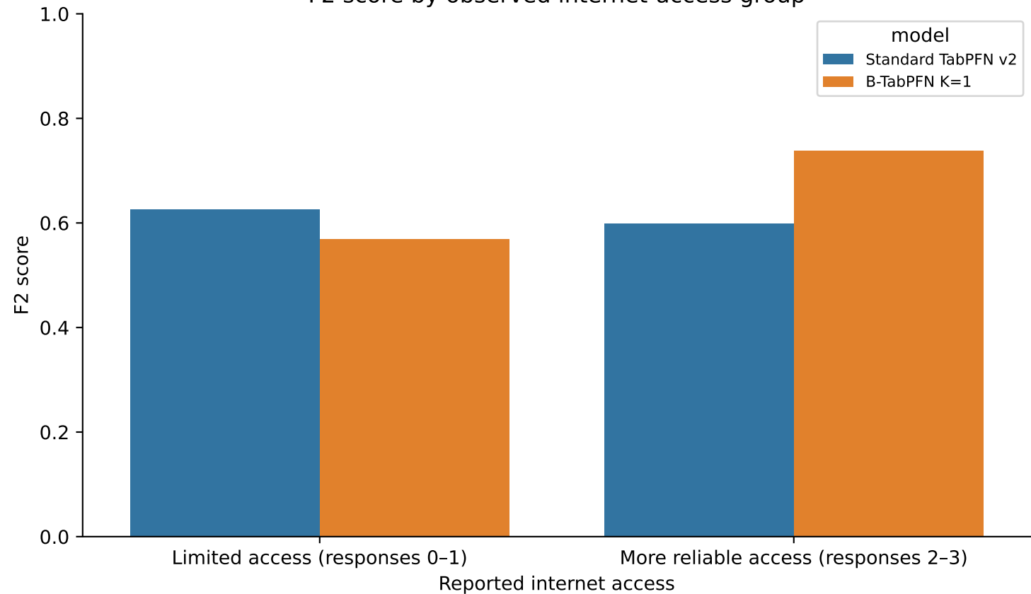
F2 score by observed internet-access group
