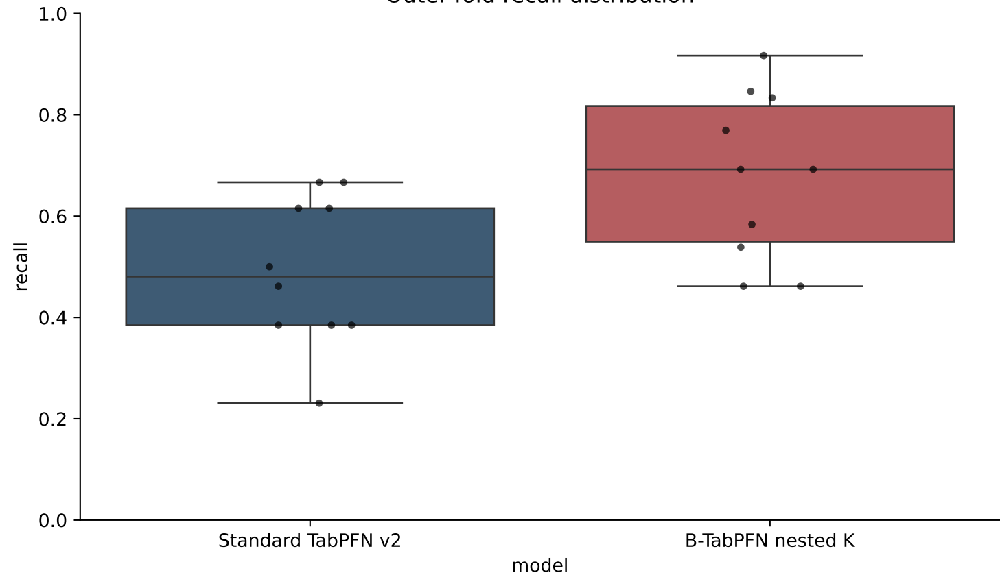
Outer-fold recall distribution
