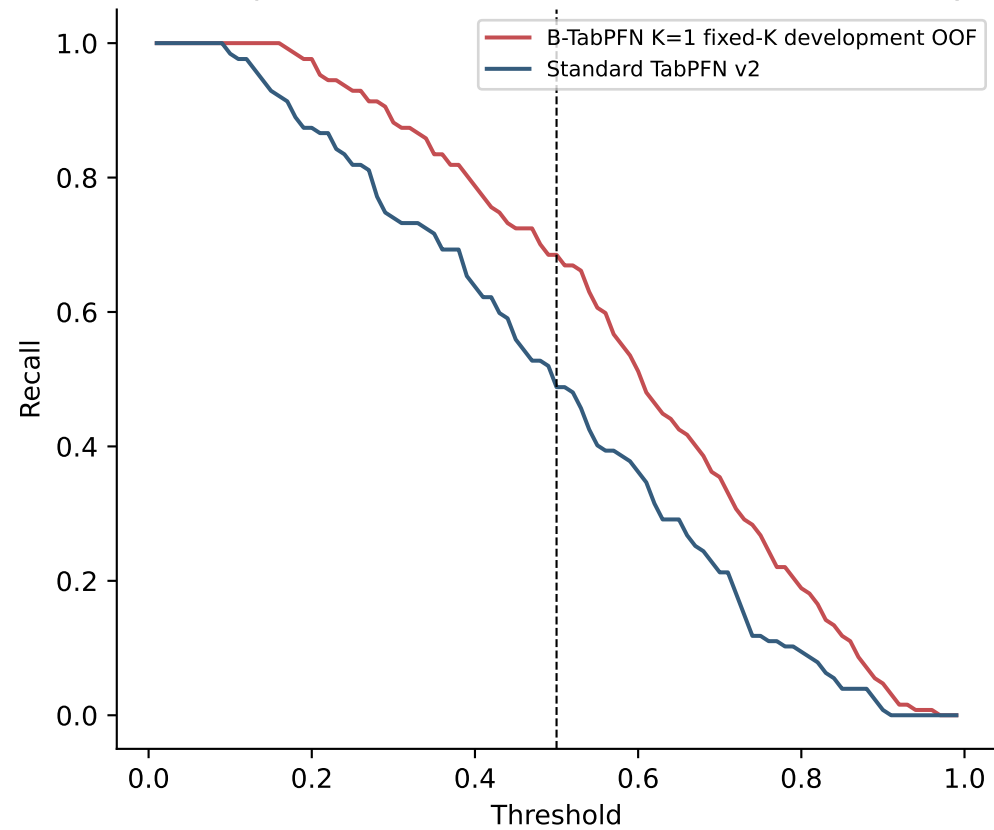
Development out-of-fold Recall threshold sensitivity
