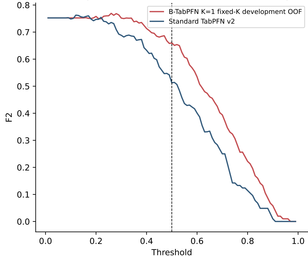
Development out-of-fold F2 threshold sensitivity
