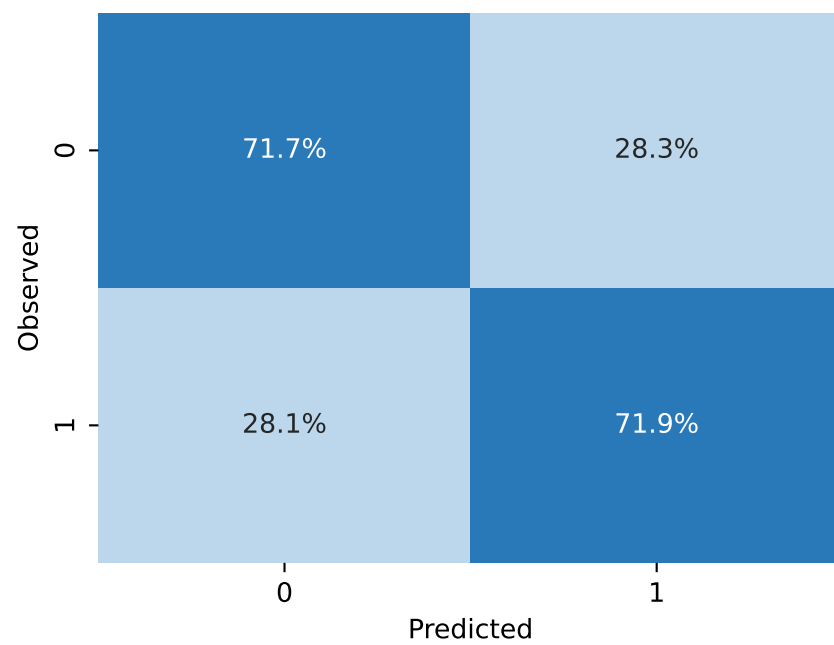
B-TabPFN K=1 — row-normalized
