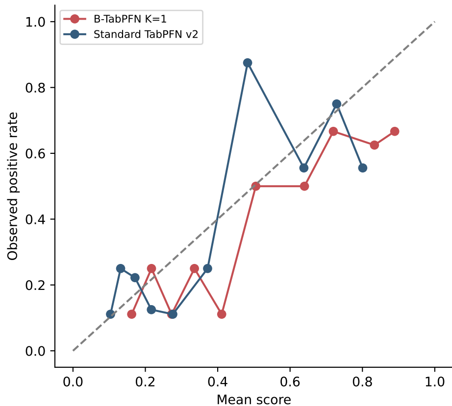
Held-out test
