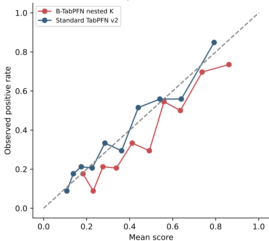
Development out-of-fold
