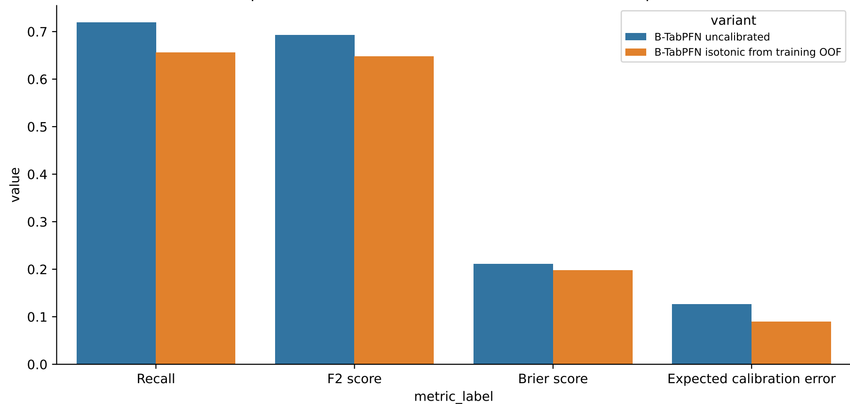
Development-fitted isotonic recalibration on the held-out partition
