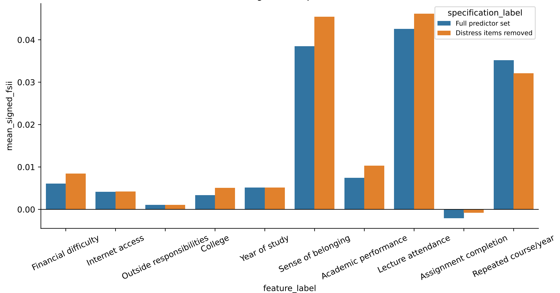
Attribution shift after removing distress predictors—not causal mediation
