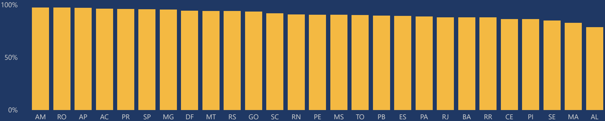
On Time Delivery Rate by State
