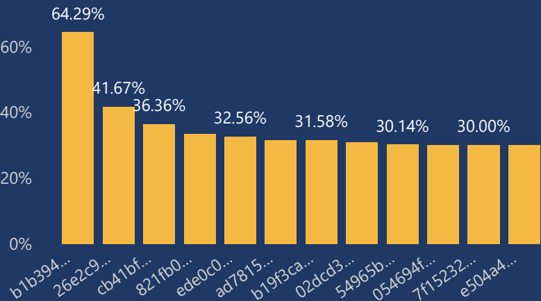
Worst Sellers by Delivery Rates
