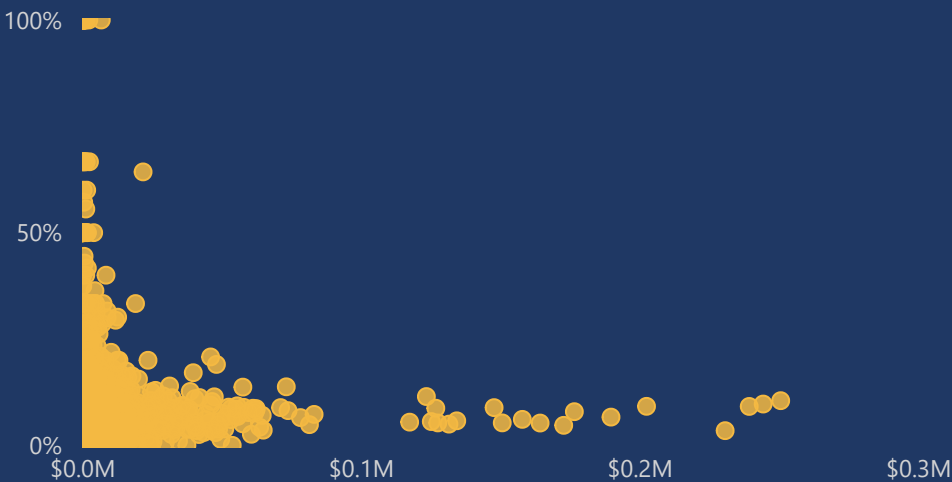
Total Revenue and Late Delivery Rate by Sellers
