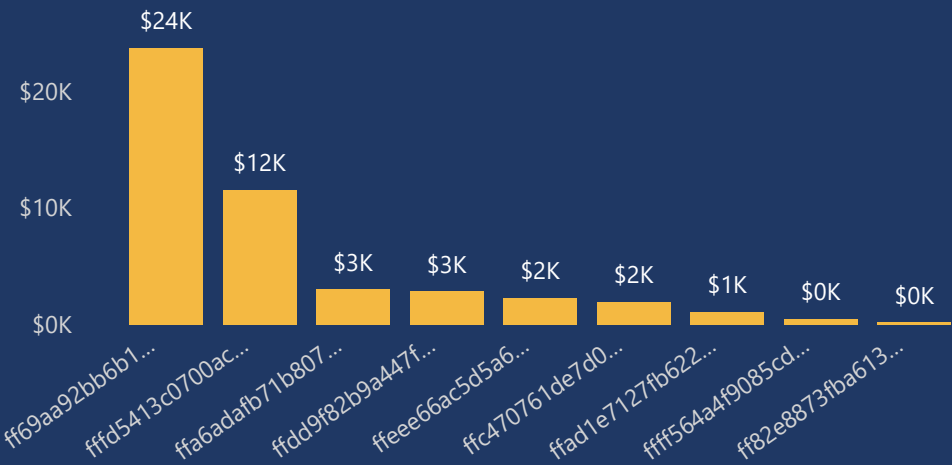
Total Revenue by Sellers
