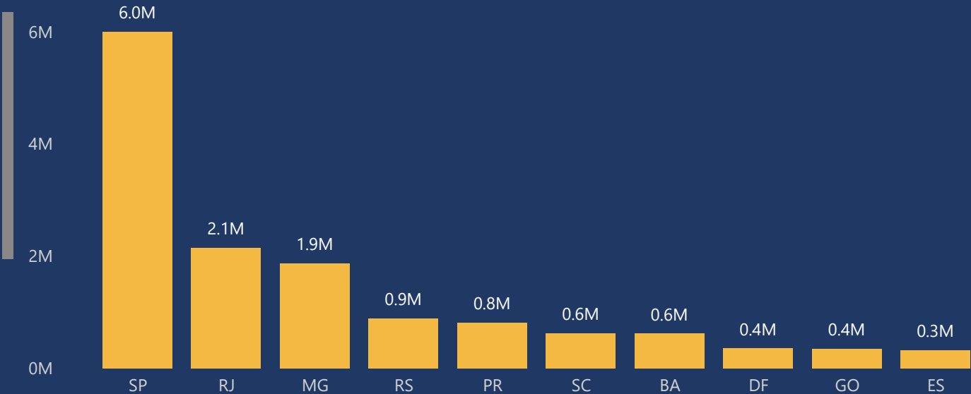
Total Revenue by State
