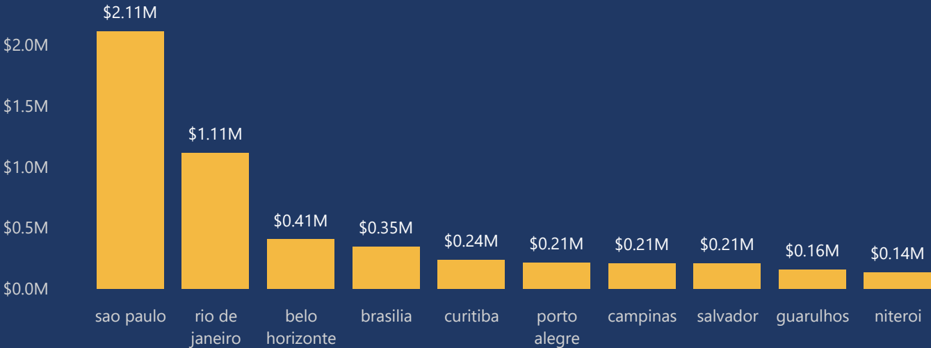
Total Revenue by City
