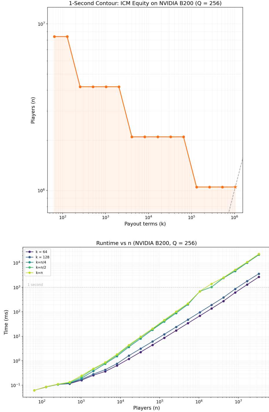
Figure 6: NVIDIA B200. Top: one-second contour (maximum n achievable within 1 s as a function of k ), the GPU analogue of Figure 1. Bottom: runtime vs. n at fixed k , showing the tree-level cliffs referenced below.
