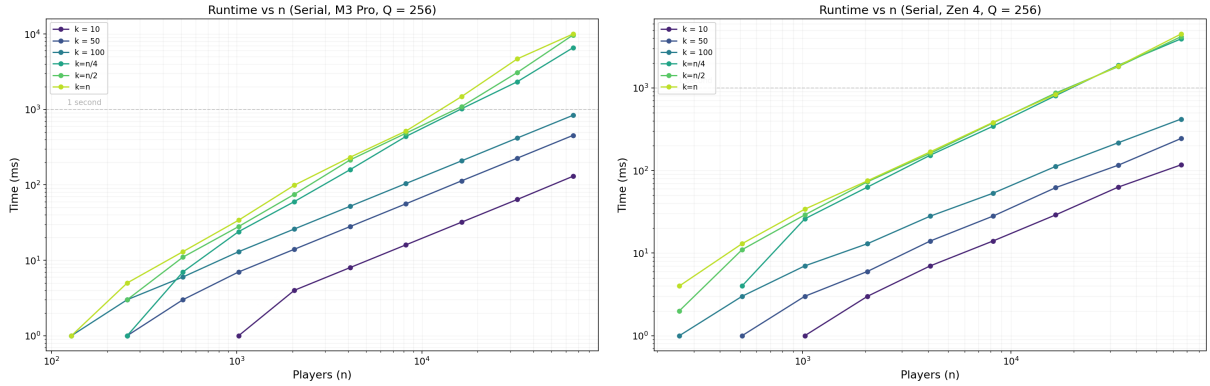
Figure 4: Runtime vs. n at fixed k , single-threaded. Left: Apple M3 Pro. Right: AMD Zen 4. The CPU analogue of the GPU runtime plot in Figure 6.
