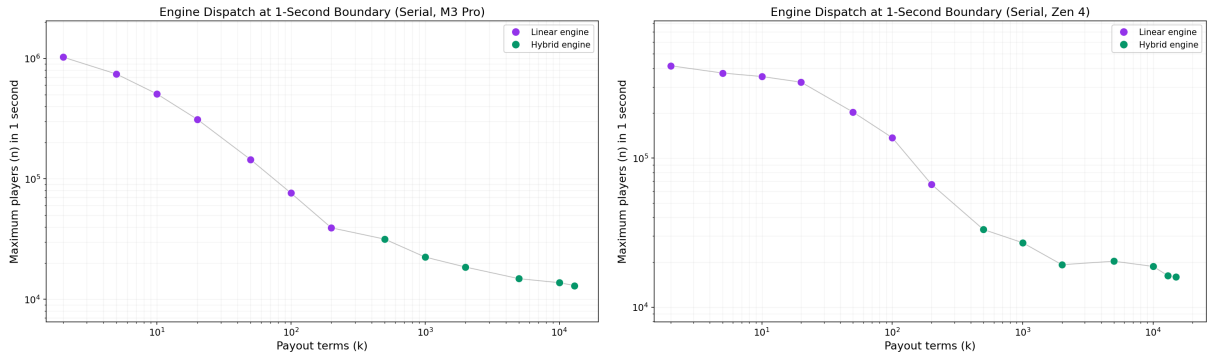
Figure 3: Engine dispatch decisions at the one-second boundary. Purple: linear engine. Green: hybrid engine. Left: M3 Pro. Right: Zen 4.
