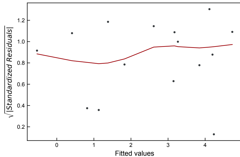
Scale-Location
