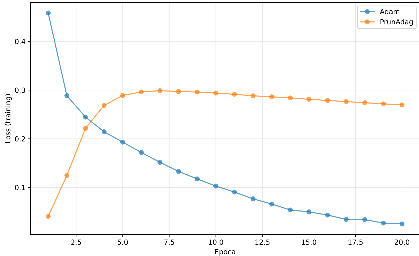
Curve di Loss: FashionMNIST + CNN
