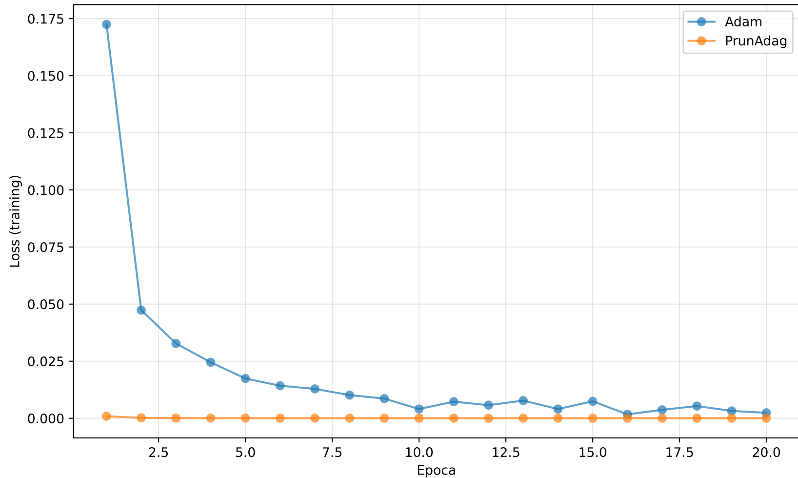
Curve di Loss: MNIST + CNN
