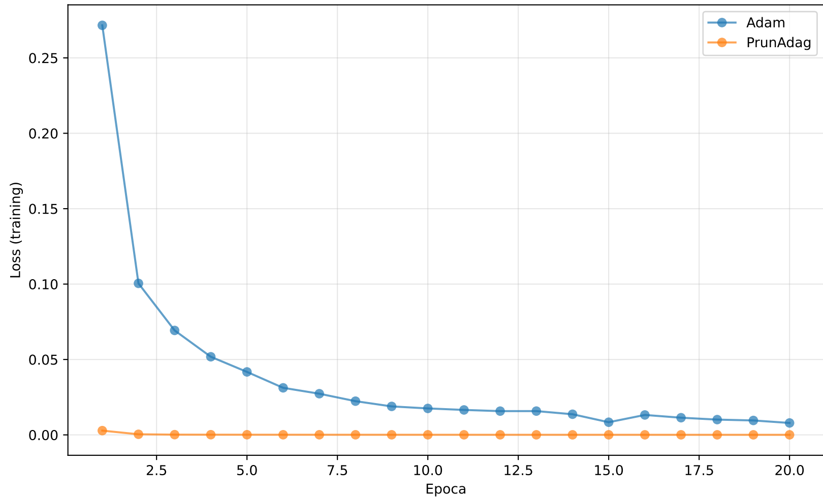
Curve di Loss: MNIST + MLP
