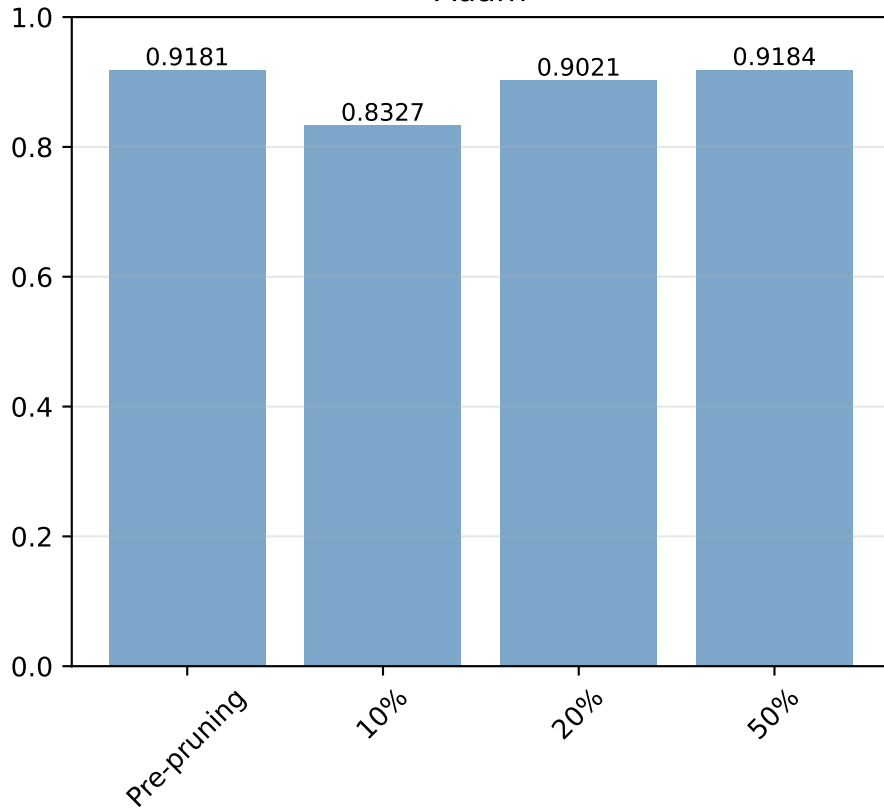
Adam
