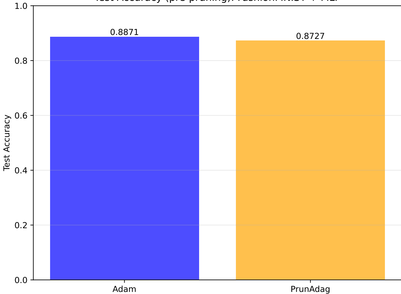
Test Accuracy (pre-pruning): FashionMNIST + MLP
