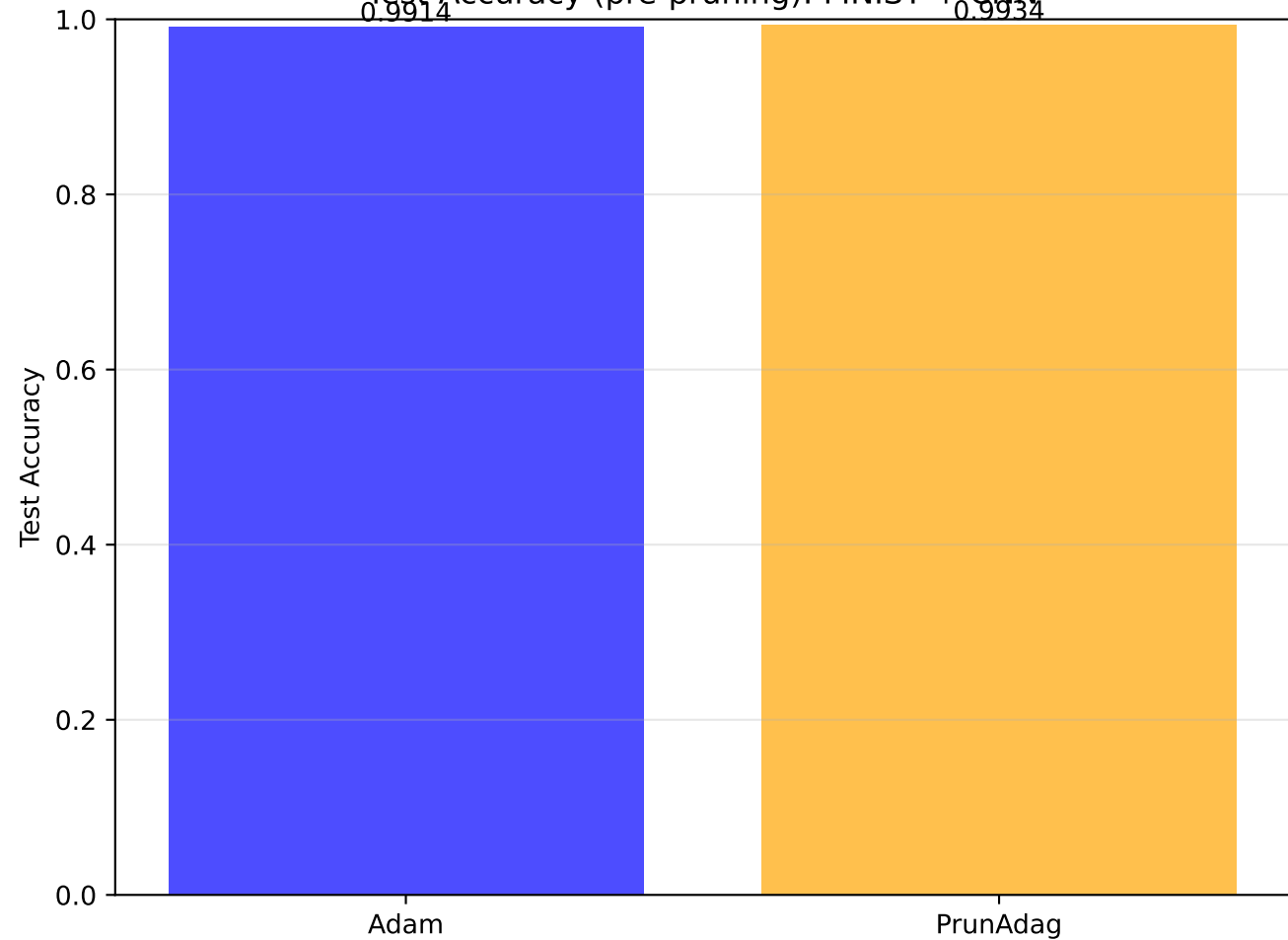
Test Accuracy (pre-pruning): MNIST + CNN
