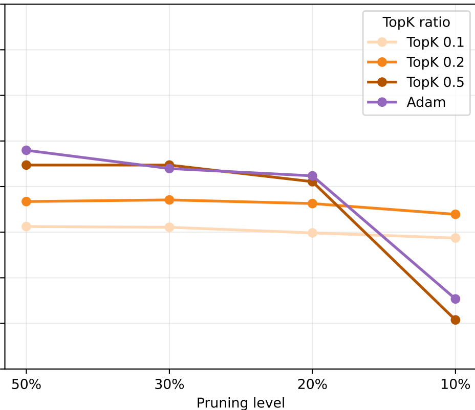
FashionMNIST | CNN
