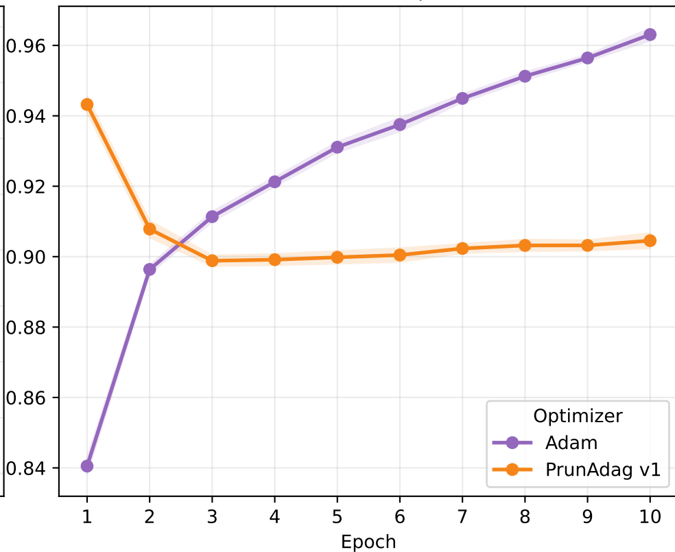
FashionMNIST | CNN
