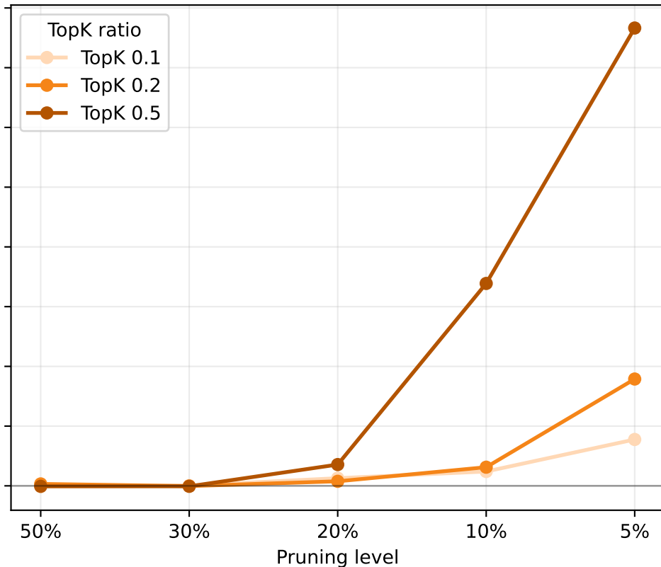
FashionMNIST | CNN
