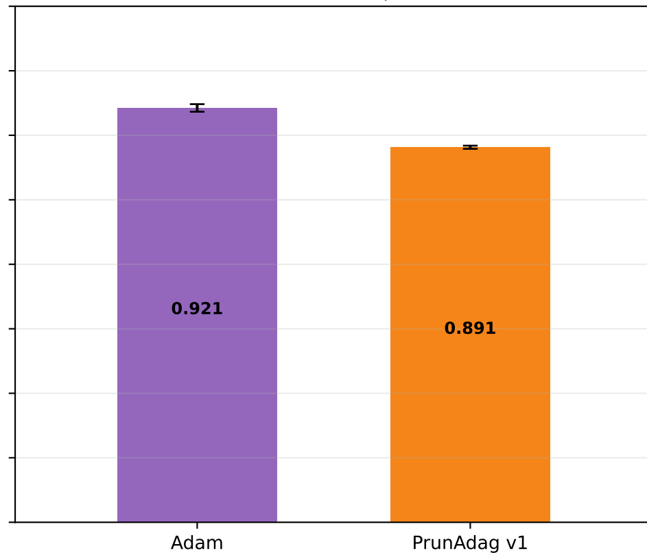
FashionMNIST | CNN
