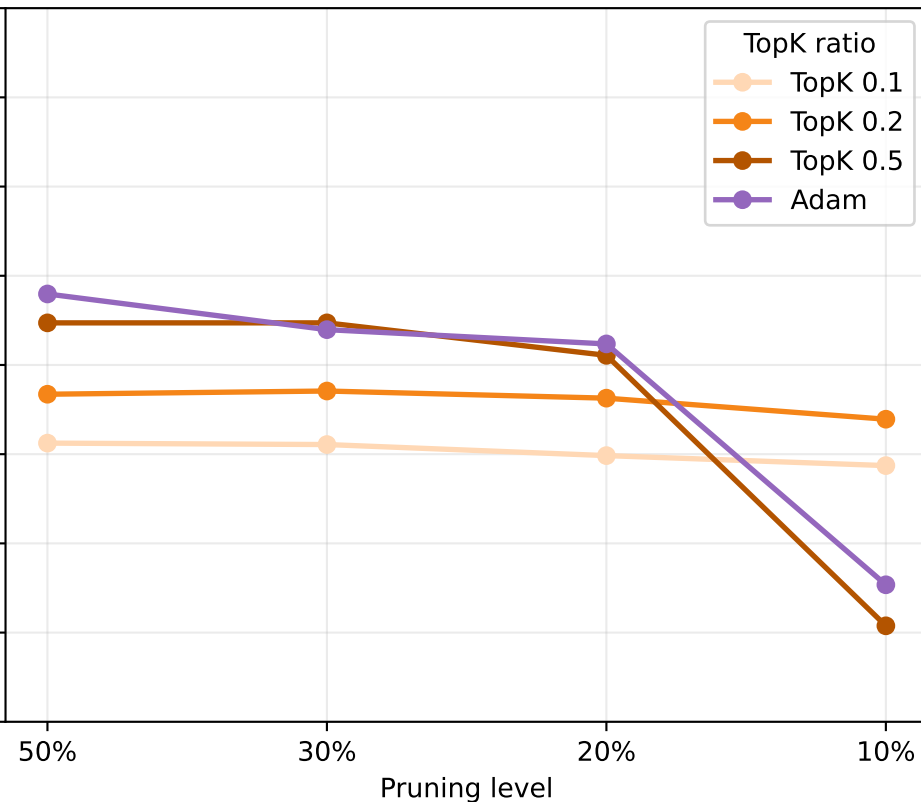
FashionMNIST | CNN
