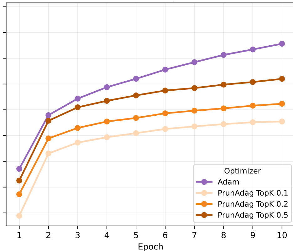
FashionMNIST | CNN
