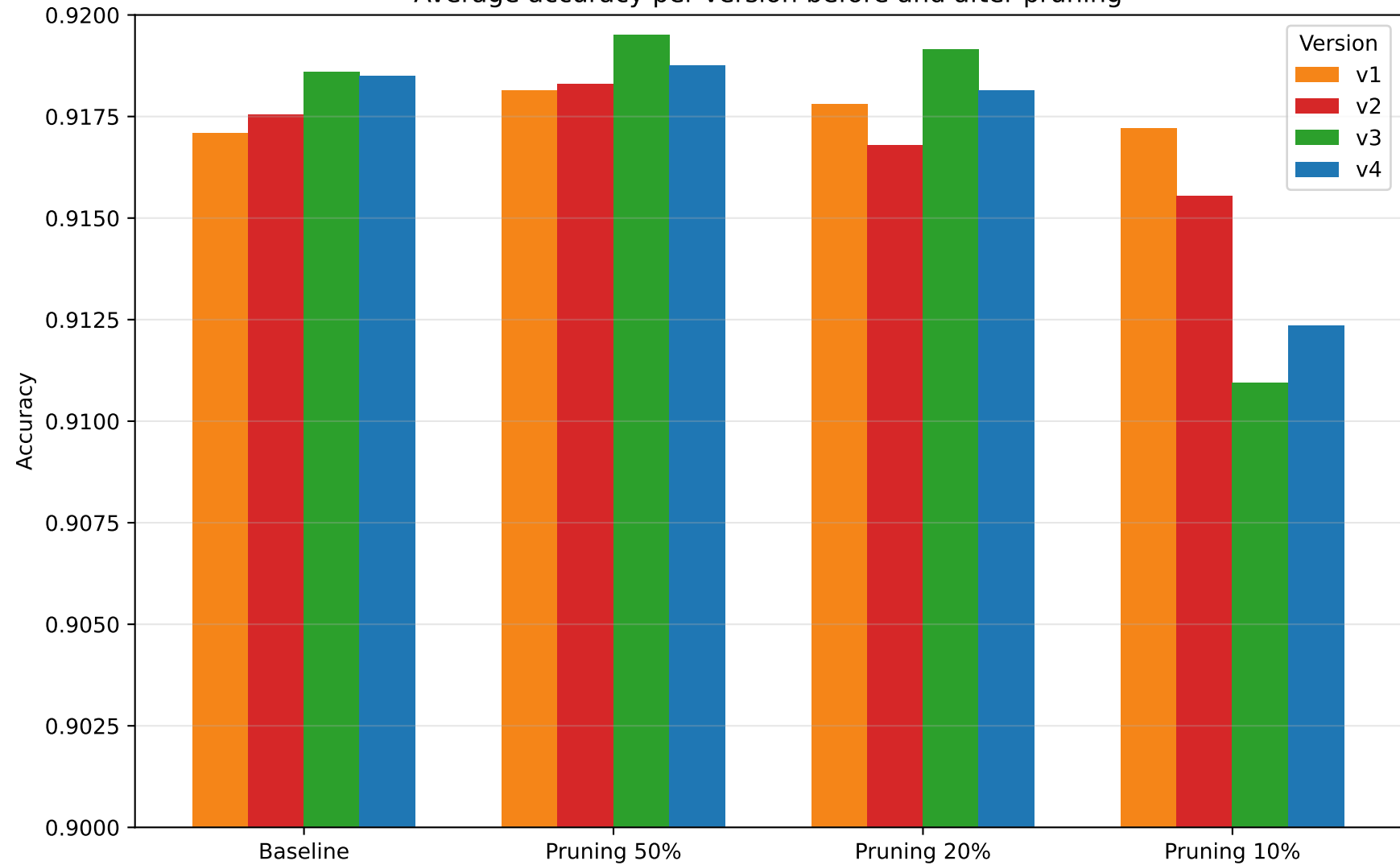
Average accuracy per version before and after pruning
