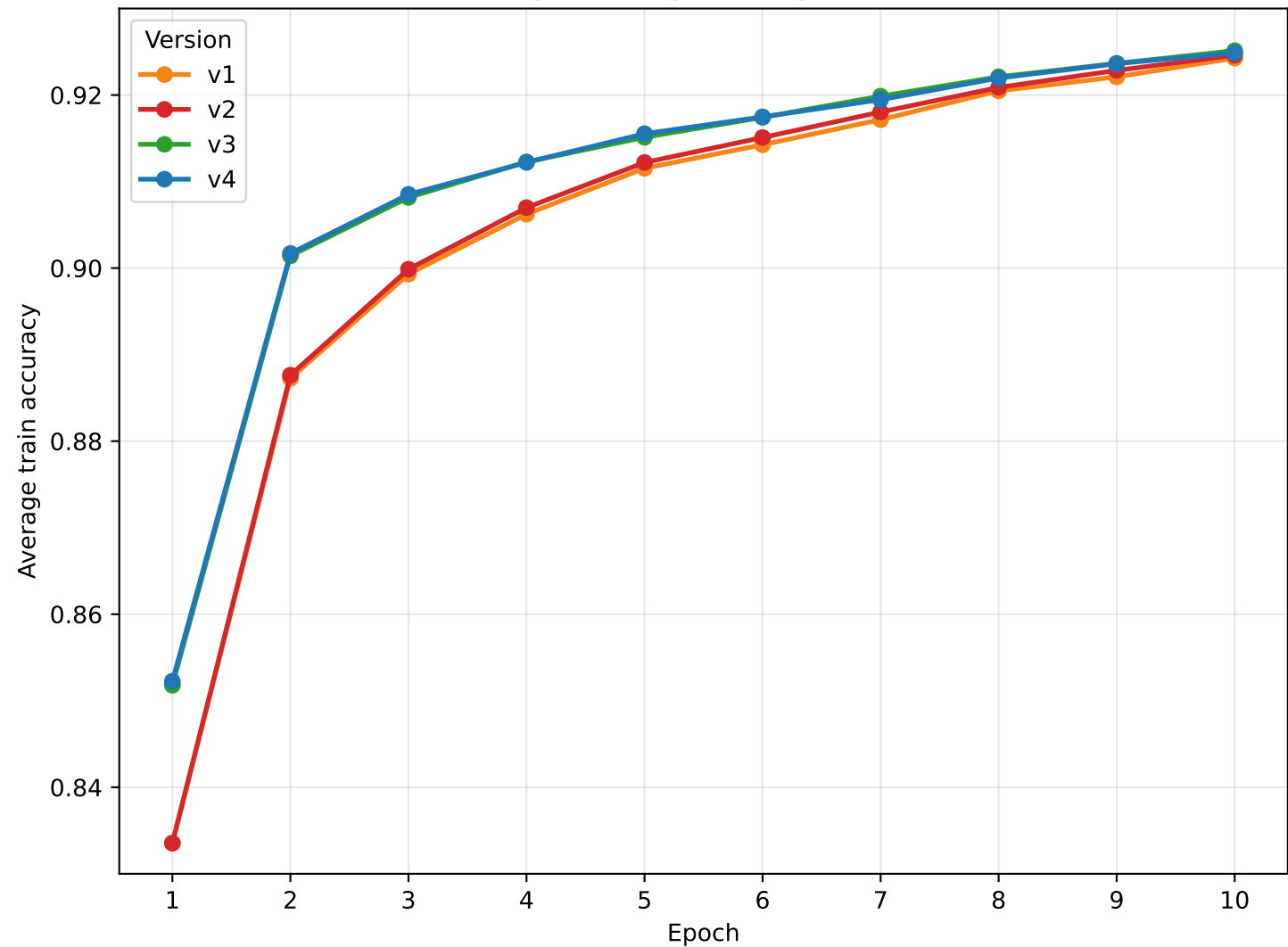
Average training curves per version
