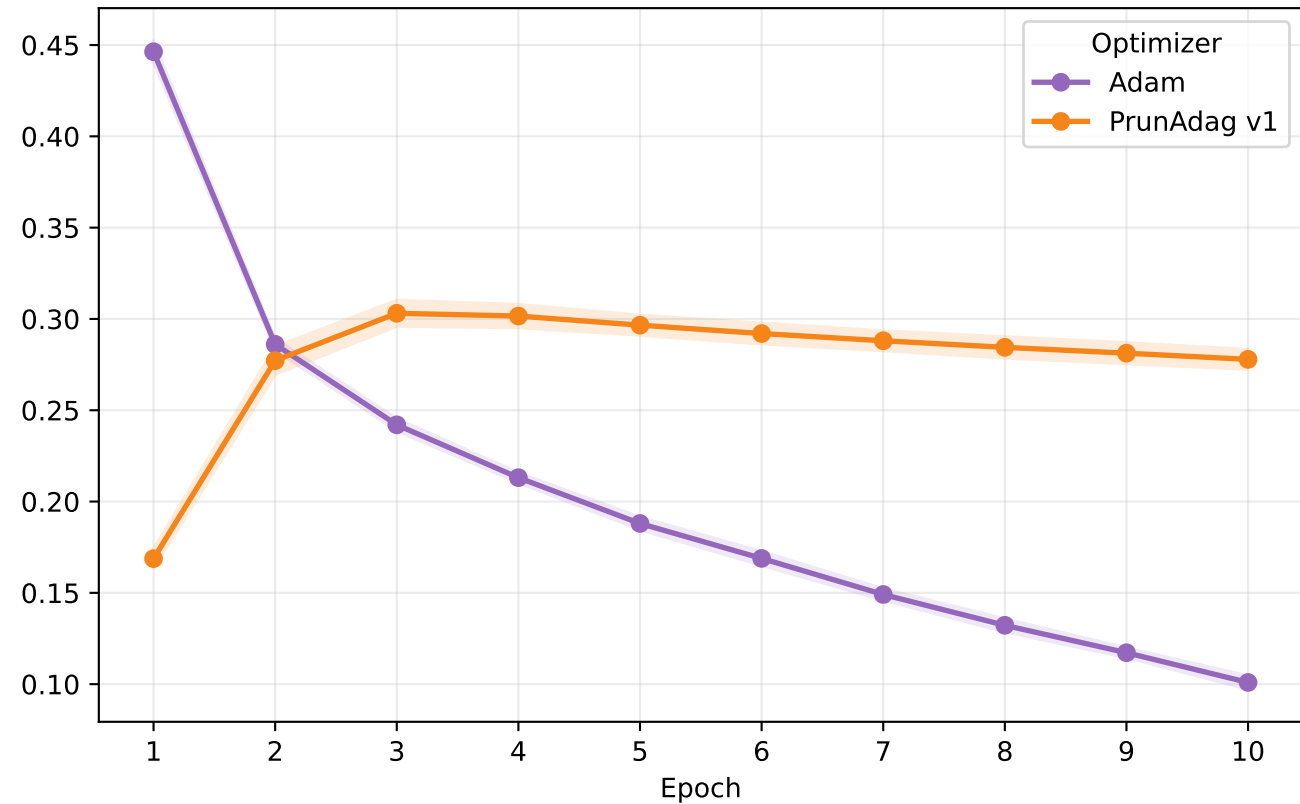
FashionMNIST | CNN
