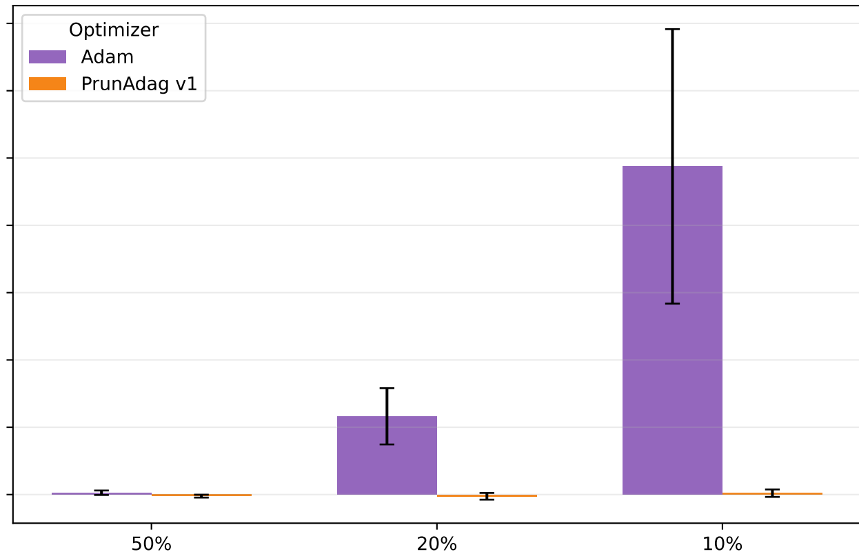
FashionMNIST | CNN
