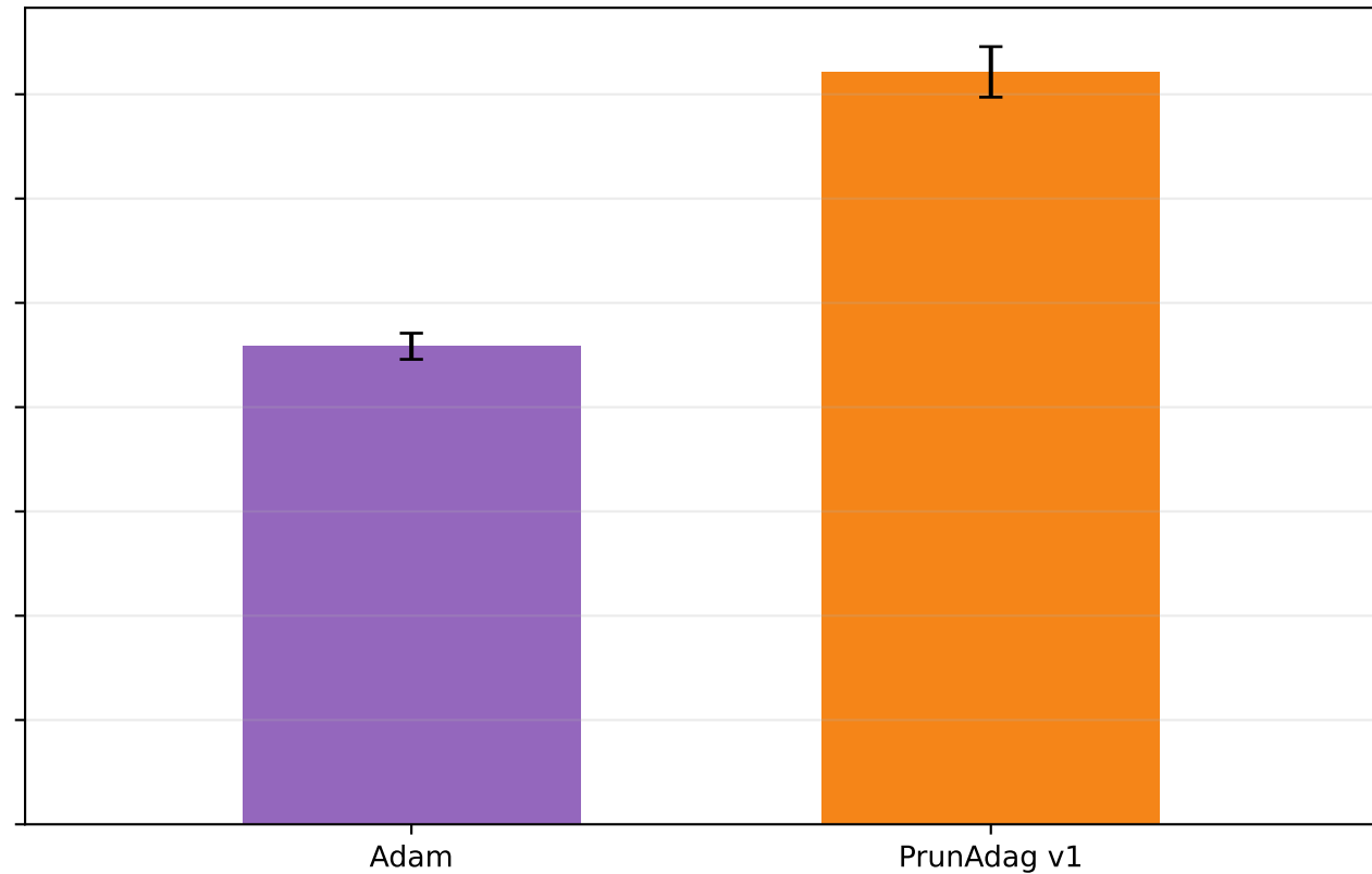
FashionMNIST | CNN
