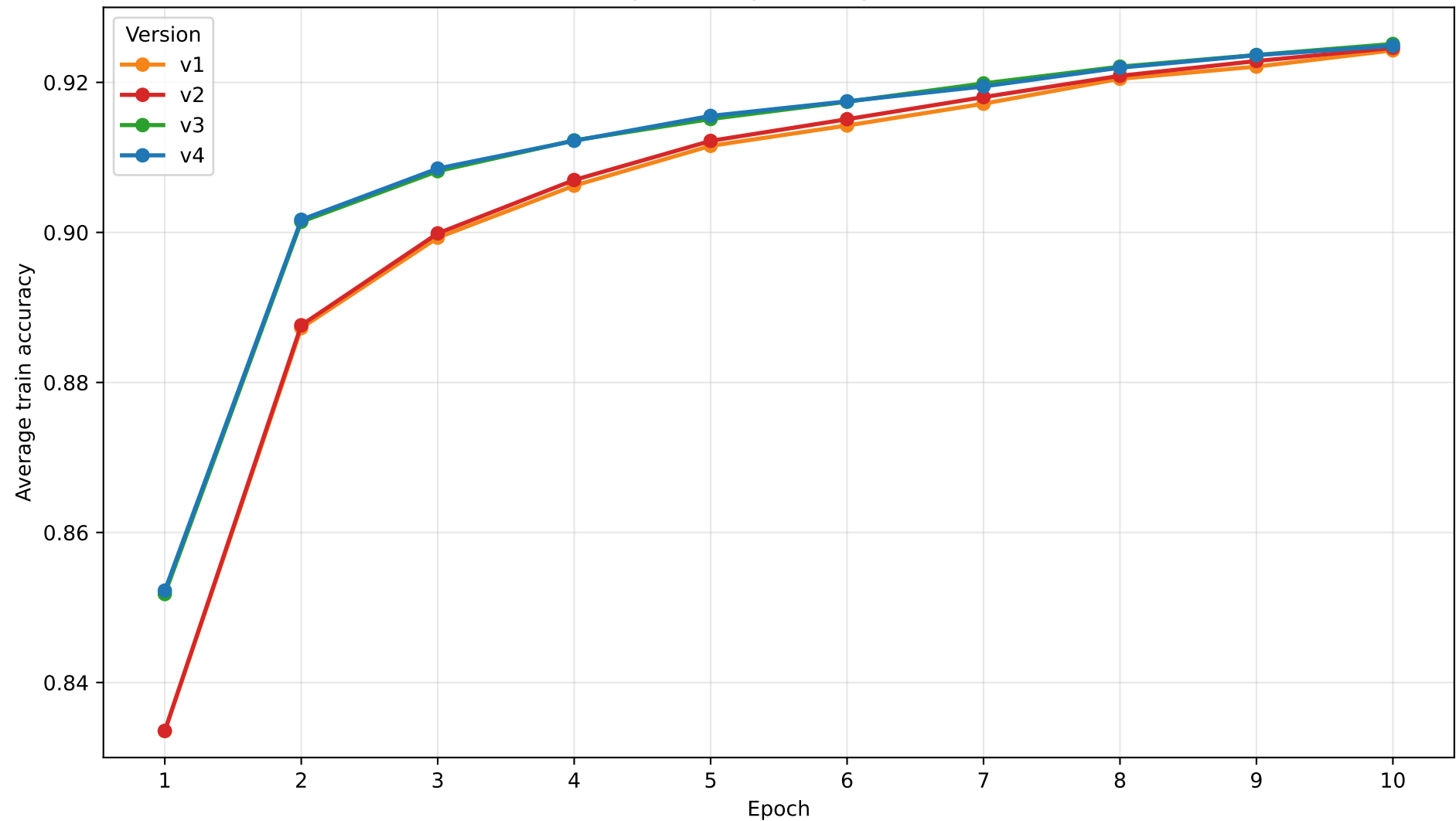
Average training curves per version
