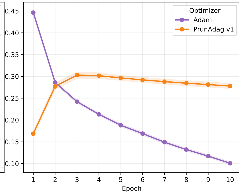
FashionMNIST | CNN
