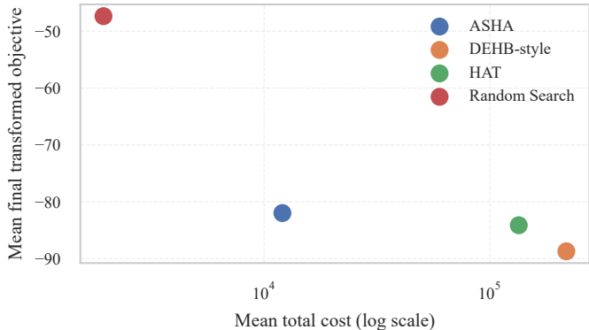
LCBench Pareto View: Cost vs Final Transformed Objective
