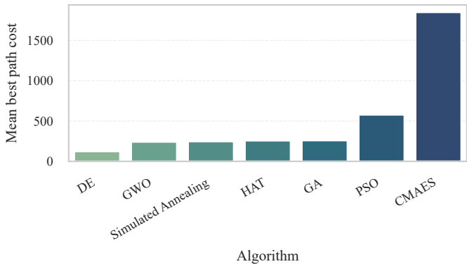
Pathfinding: Mean Best Cost by Algorithm
