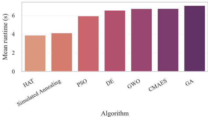
Pathfinding: Mean Runtime by Algorithm
