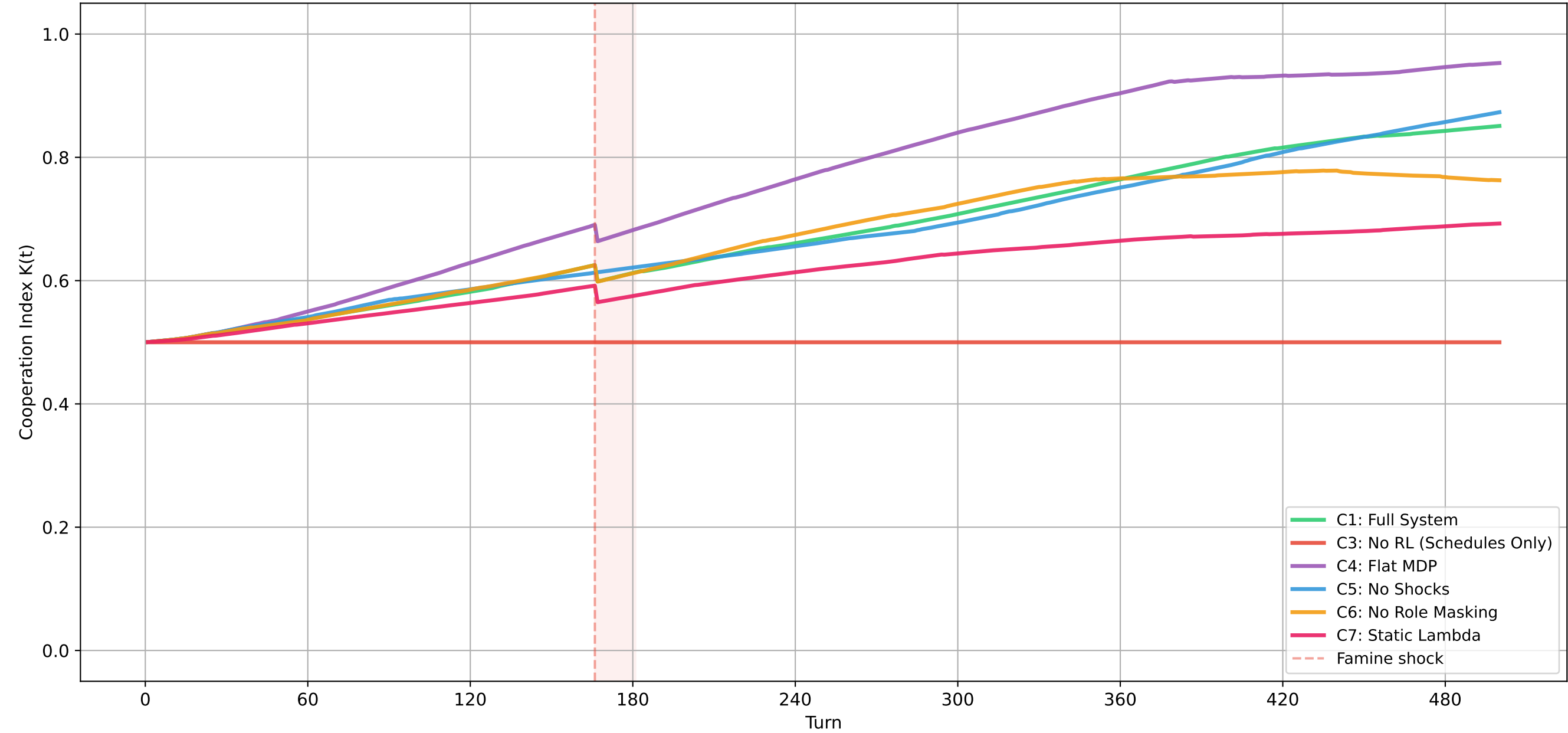
Cooperation Emergence: Ablation Comparison
