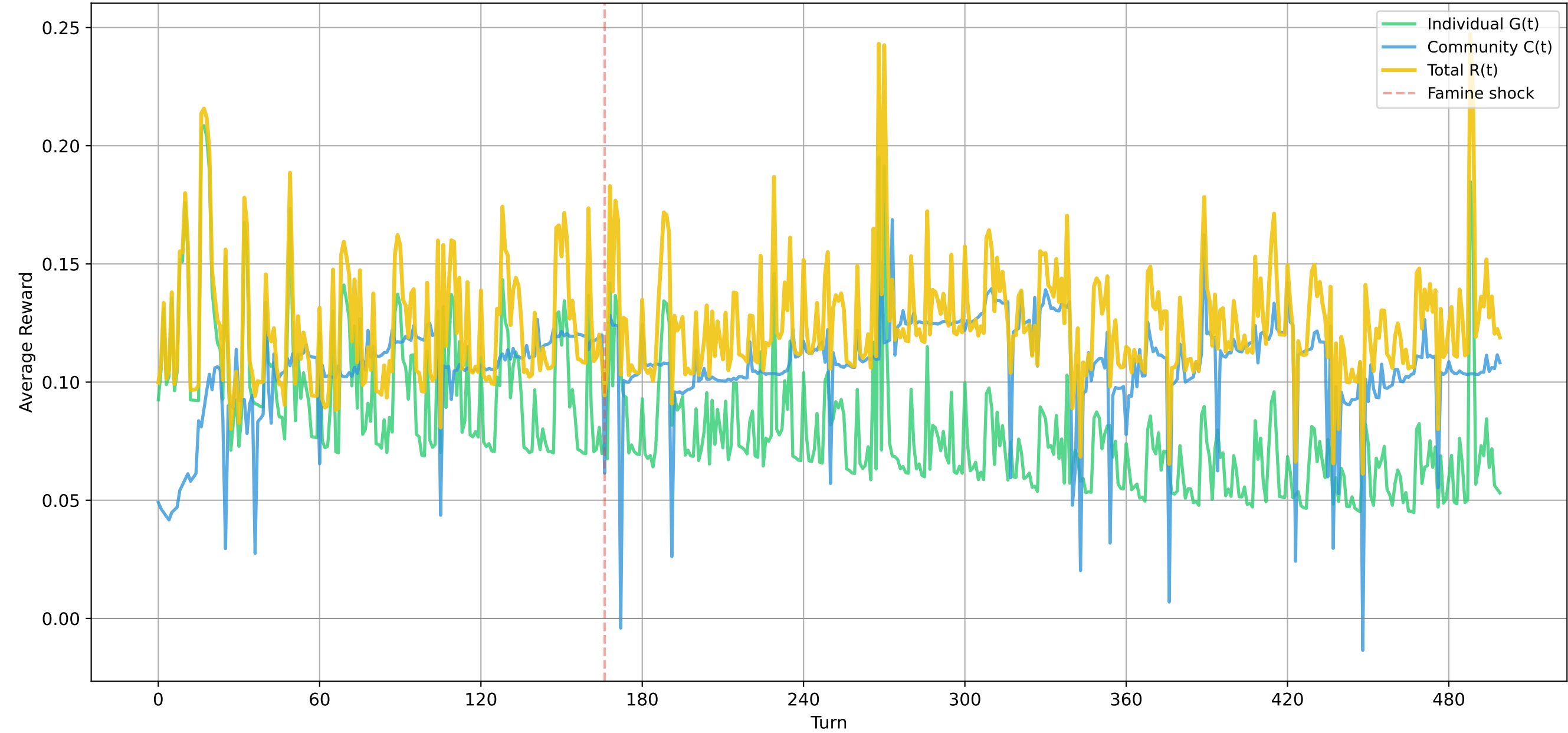
Reward Decomposition (Full System C1)
